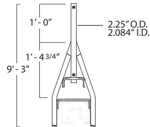
TOP SECTION 25AG3
