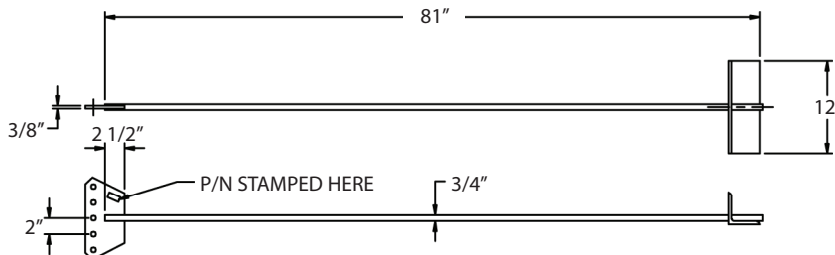
GAC3455TOP ( 17,670 LBS. ALLOWABLE LOAD)*
