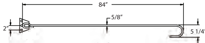
GAC303 ( 7,330 LBS. ALLOWABLE LOAD)*
