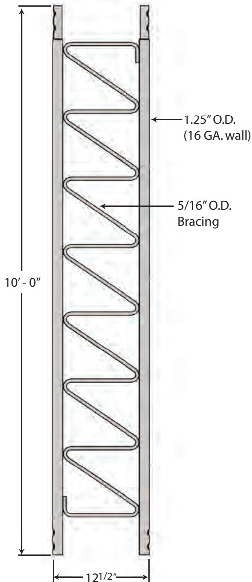
STANDARD SECTION 25G - 10' Section 25G7 - 7' Section
