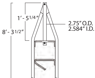
TOP SECTION 25AG5
