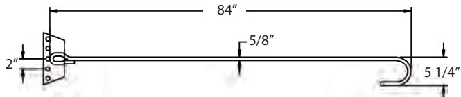
GAC305 ( 7,330 LBS. ALLOWABLE LOAD)*
