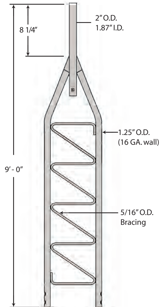
STANDARD TOP SECTION 25AG
